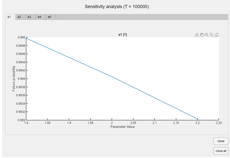
Figure 23: Sensitivity analysis of the modified highway pilot model from figure 21. All parameters have been varied with \pm 10\% .
