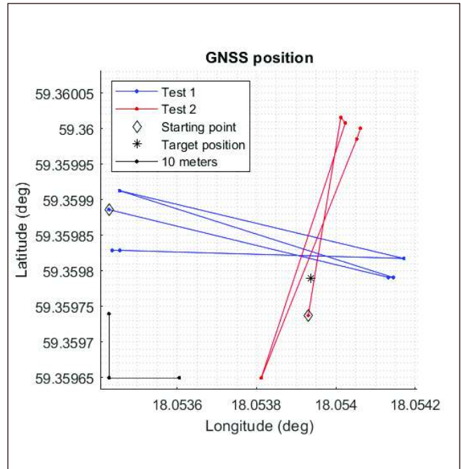
Results from dynamic positioning tests.
