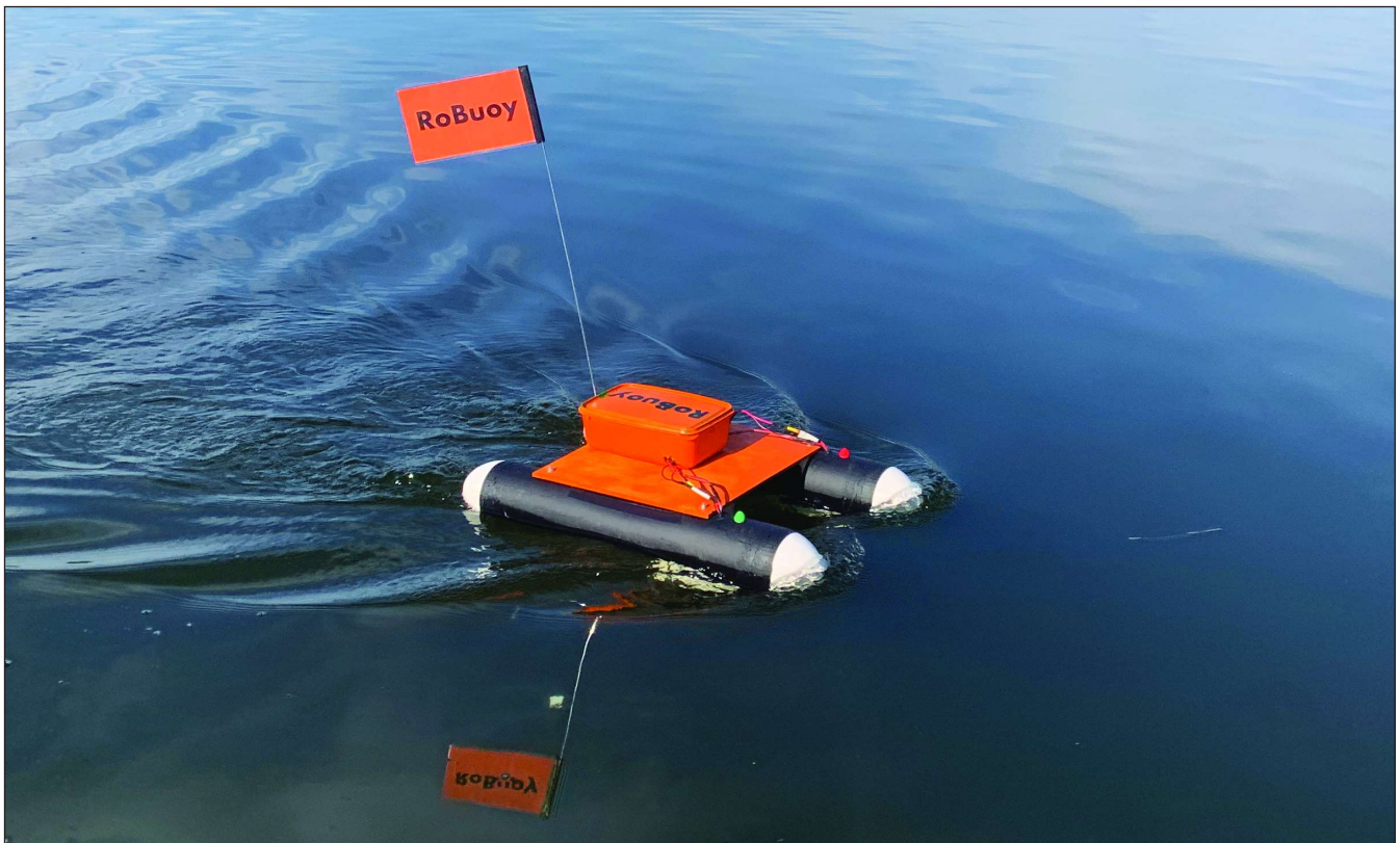
RoBuoy on its way to a target position, autonomously navigating using a GNSS-receiver, a compass and electric motors.
