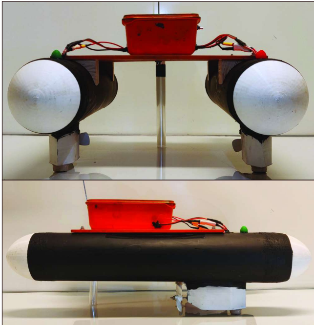
Front view and side view of RoBuoy.
