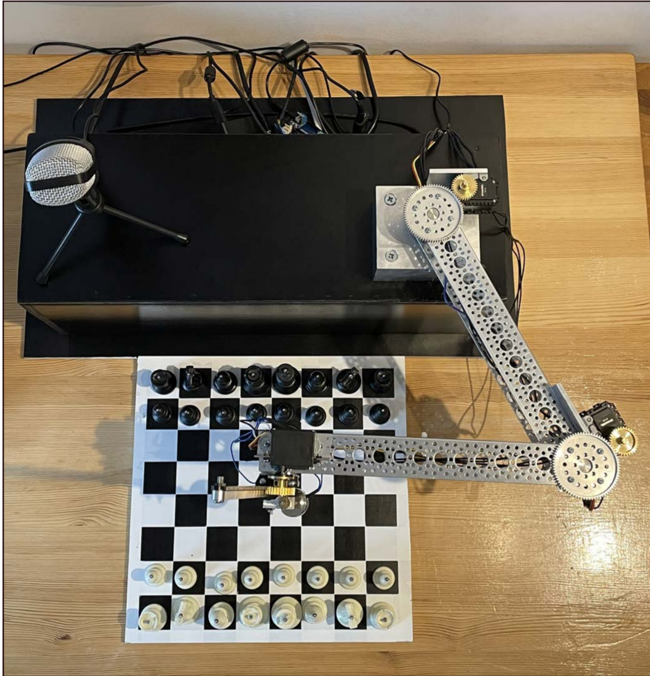
Chess robot as seen from above.
