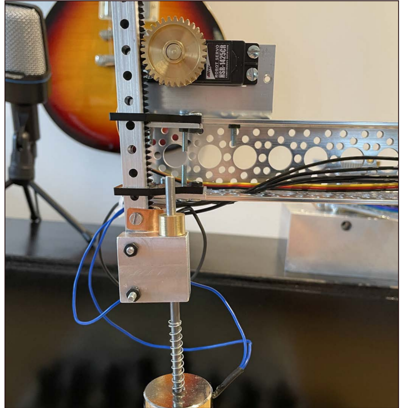
RC Servo and electromagnet for picking up chess pieces.
