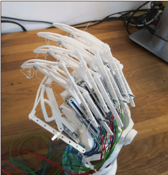
Side view of the exosksleton.
