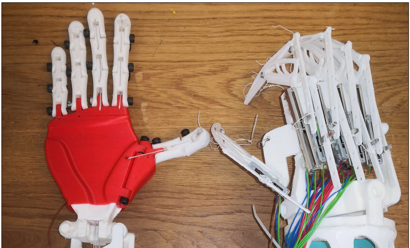
Robotic hand and exoskeleton side by side.
