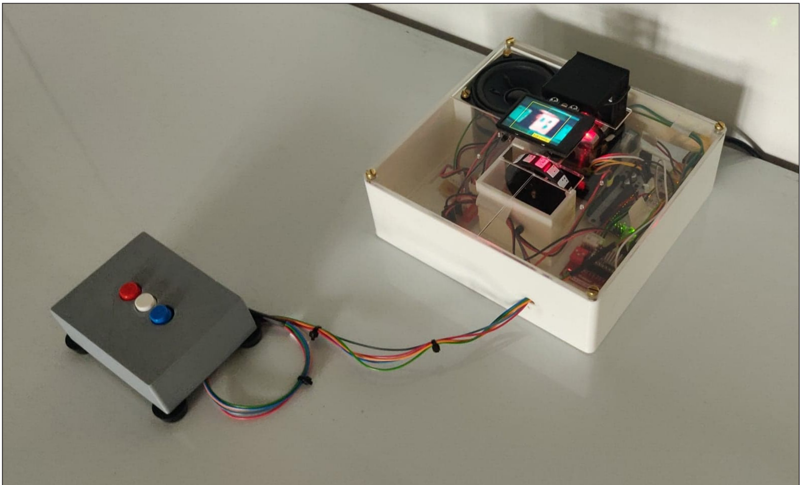
An overall picture showing the final construction of The Brailled. The instrument translates the letters of Braille into voice messages. The keyboard controls all operations.
