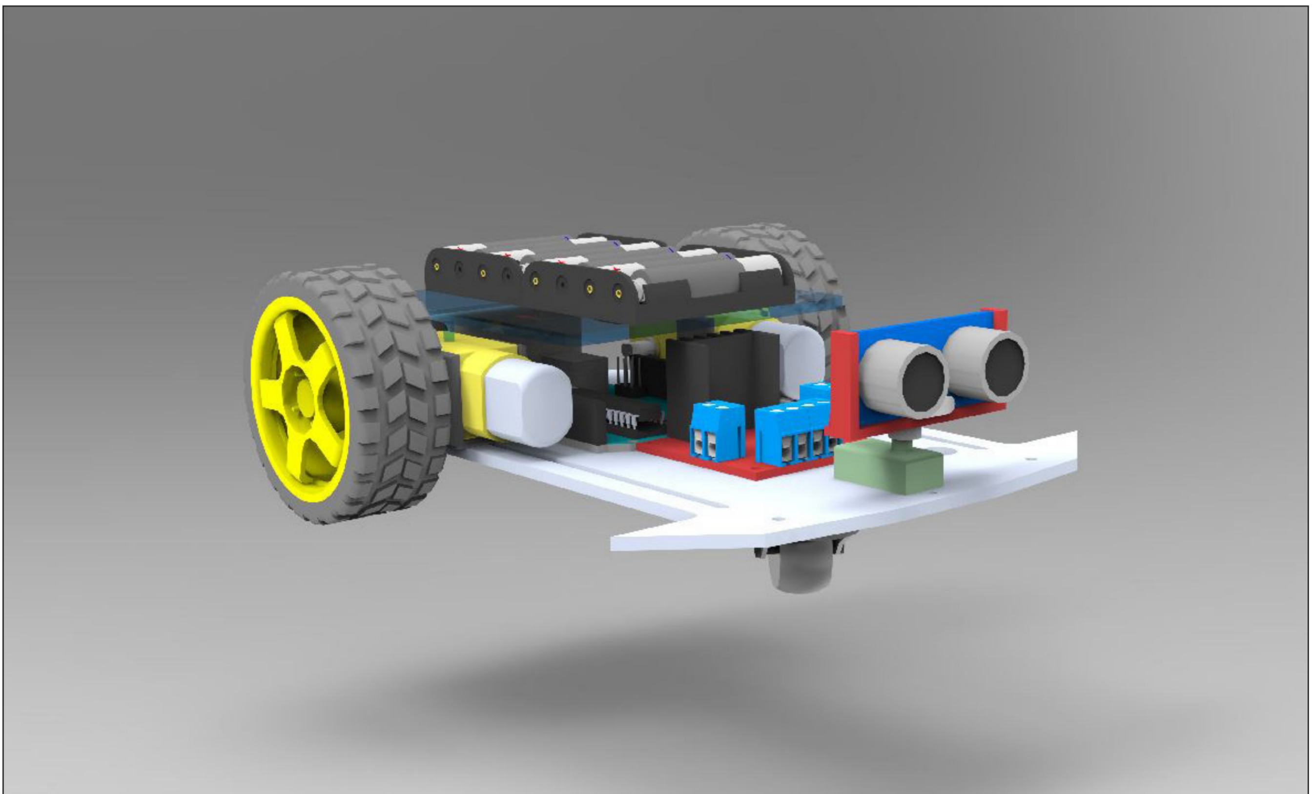
A 3D-model of the prototype of a robot that sweeps a tennis court and it's white lines by itself.
