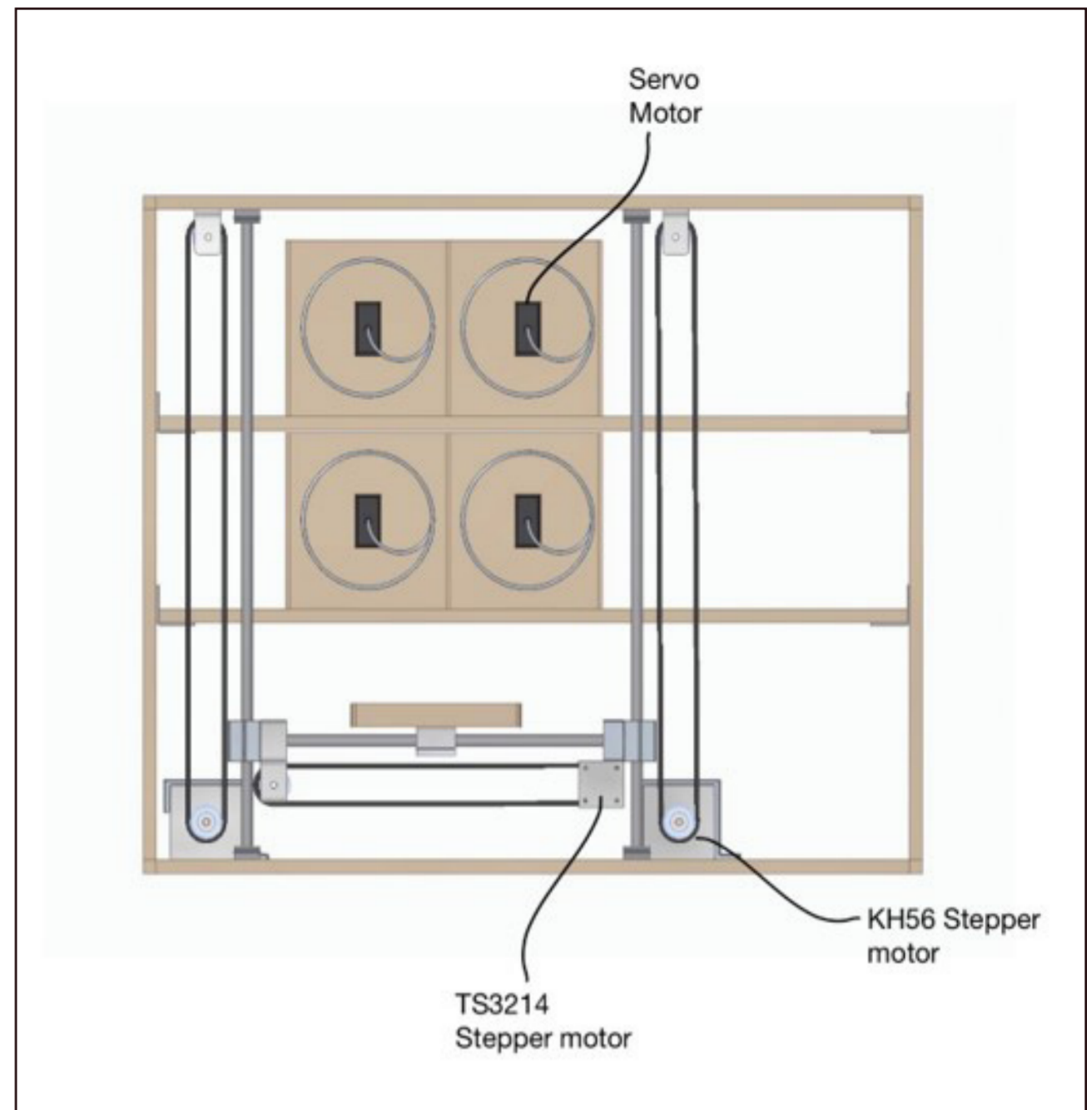
CAD model of the internal frame of the prototype.
