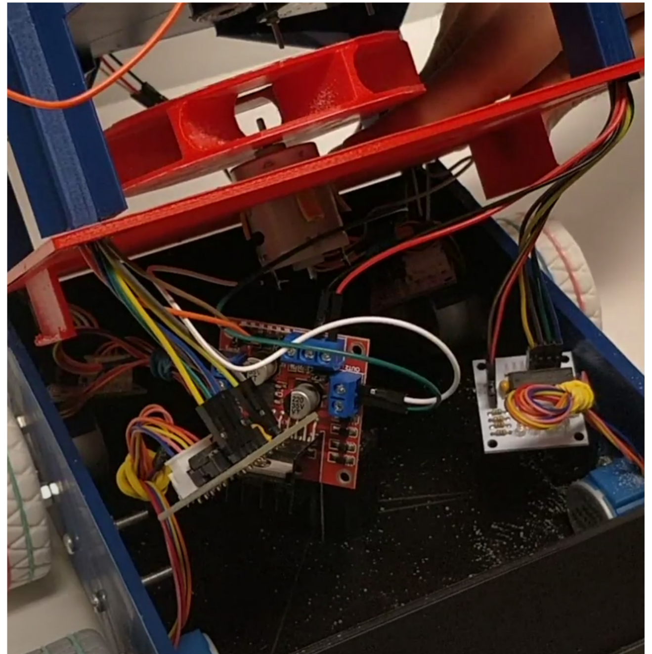
The wheels are driven by four Stepper motors and the rotor is driven by a DC motor.
