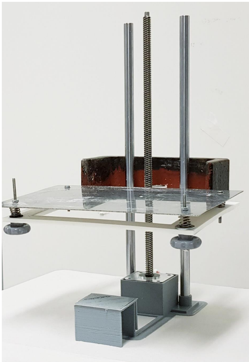
The print bed and Z-axis assembly
