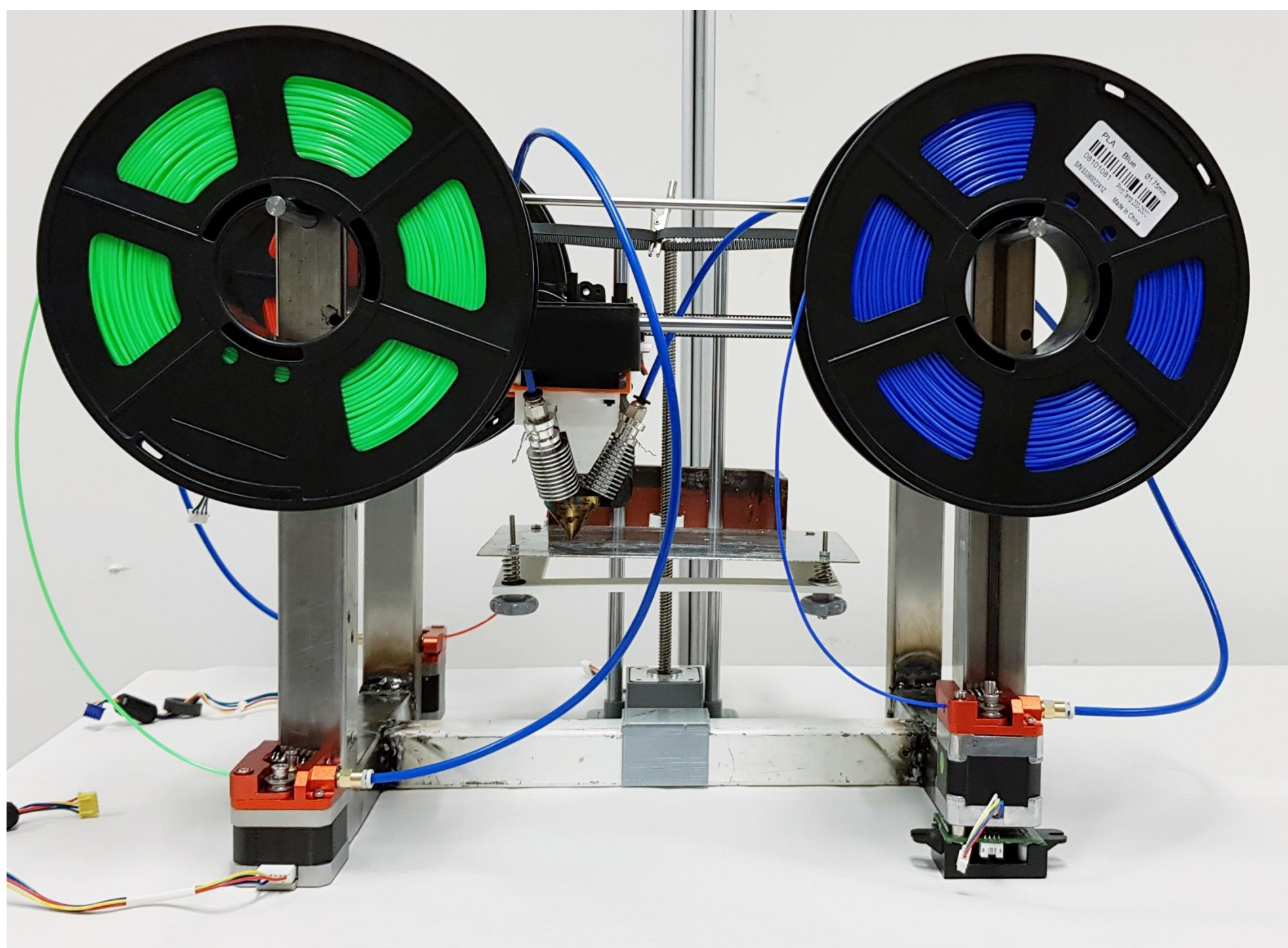
The final prototype before wiring and it can print 24 distinct colors
