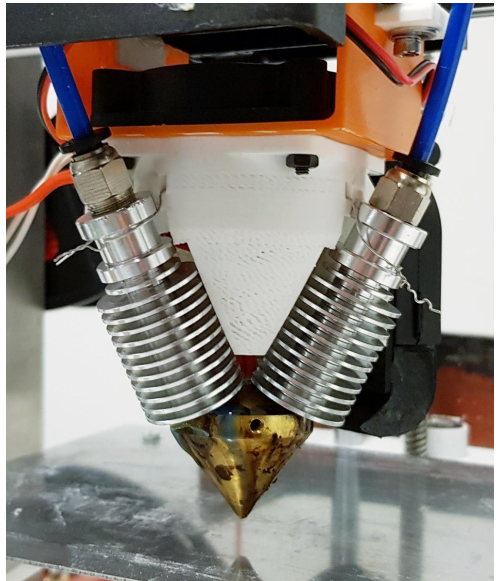
Diamond Hotend
