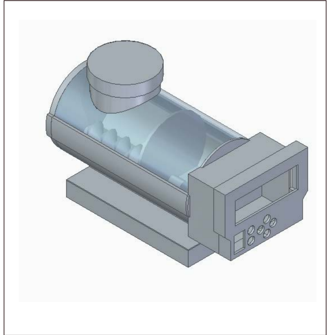
CAD design of fish feeder with visible internals
